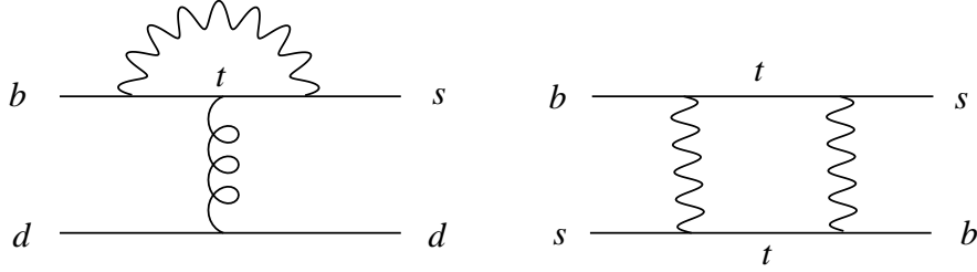
FIG. 3. Penguin diagram (left) and box diagram (right).
